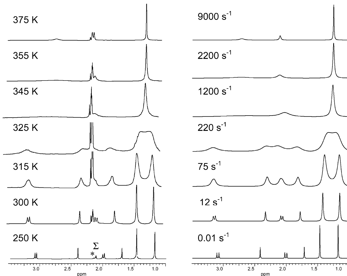
Figure 9. Experimental (left) and simulated (right) variable-temperature ^1\text{H} NMR spectra of \{\text{ONOMe}\}\text{Zr}(\text{CH}_2\text{Ph})_2 ( 8 ) showing the \text{NCH}_2\text{CMe}_2 ( \delta 3.15 and 2.00), \text{ZrCH}_2\text{Ph} ( \delta 2.35 and 1.75), and \text{CMe}_2 ( \delta 1.45 and 1.15) resonances (toluene- d_8 , 400 MHz). The vertical expansion is different in each case for clarity. Best-fit first-order rate constants ( k ) are shown with the simulated spectra. The markers * and \Sigma denote resonances for \text{PhCH}_3 and \text{PhCHD}_2 , respectively.
