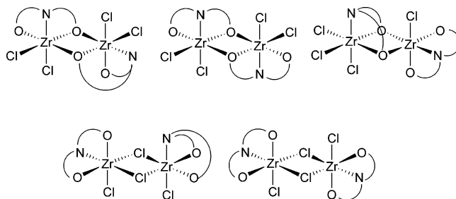
Figure 12. Schematic representations of some plausible dinuclear structures for 9 .
