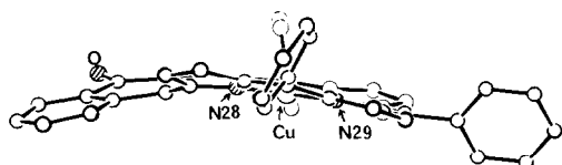
Fig. 2. The conformation of the fused benzocyclohexenone ring with respect to the porphyrin skeleton of (VI).
