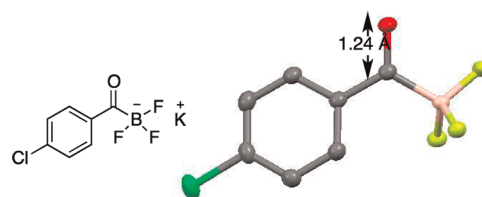
Figure 2. X-ray crystal structure of acyltrifluoroborate 5c .
