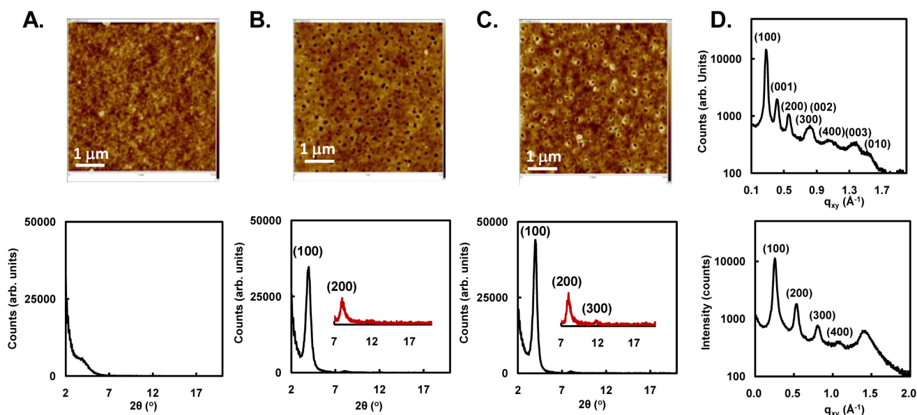
Figure 2. (A) Tapping mode AFM images ( 5 \times 5 \mu\text{m} ) and out-of-plane XRD scans of spin-coated P3 thin films without annealing; (B) after annealing at 200^\circ\text{C} ; (C) after annealing at 240^\circ\text{C} ; and (D) in-plane (top) and out-of-plane (bottom) grazing incidence X-ray scattering of spin-coated P3 thin films after annealing at 240^\circ\text{C} .
