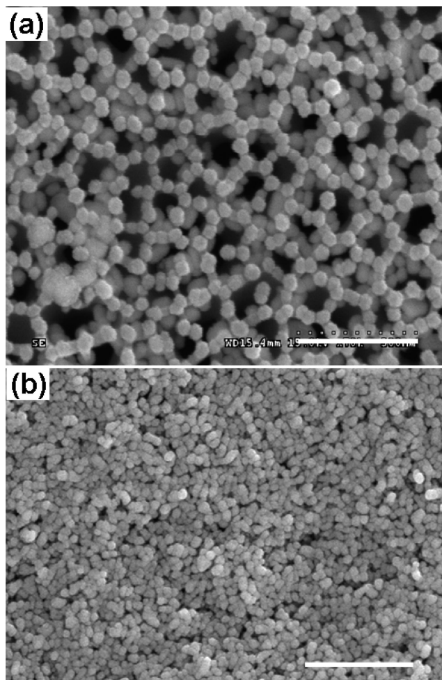
Figure 2. SEM characters of the net-like assembled colloidal Au nanoparticles on 200 nm pores of AAO membrane (a), and particle-coatings on 20 nm pores of alumina membrane (b) via the pressure difference method: the dimension bar is 500 nm for all.
