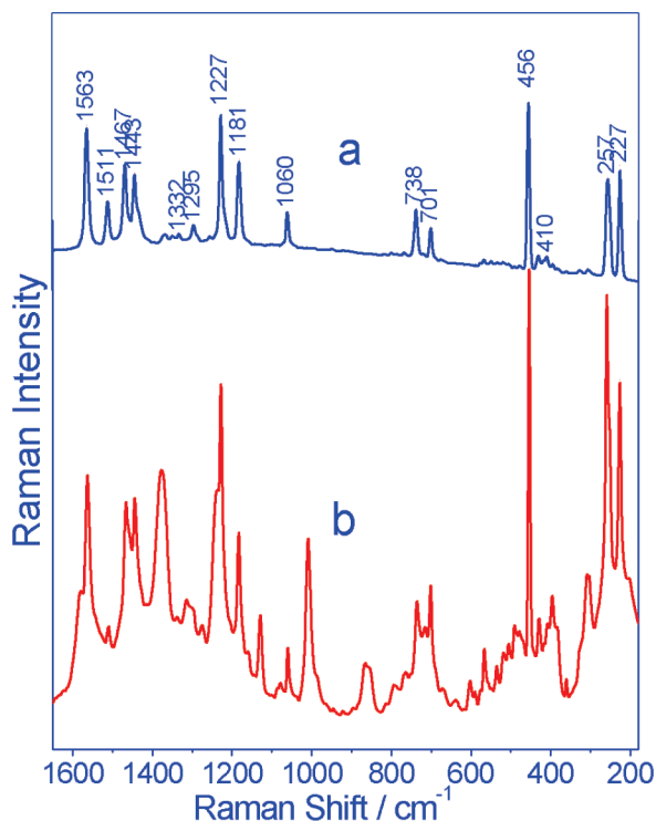
Figure 4. FT-Raman spectrum of solid fullerene C 70 (a) and SERS spectrum of C 70 from the net-assembled Au nanoparticles (b).
