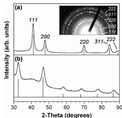
Figure 2. Powder XRD patterns for representative (a) Rh nanocrystal precursors (PDF card no. 5-0685) and (b) Rh 2 P products (PDF card no. 77-0300). A representative SAED pattern for the Rh nanocrystal precursors is shown in the inset.
