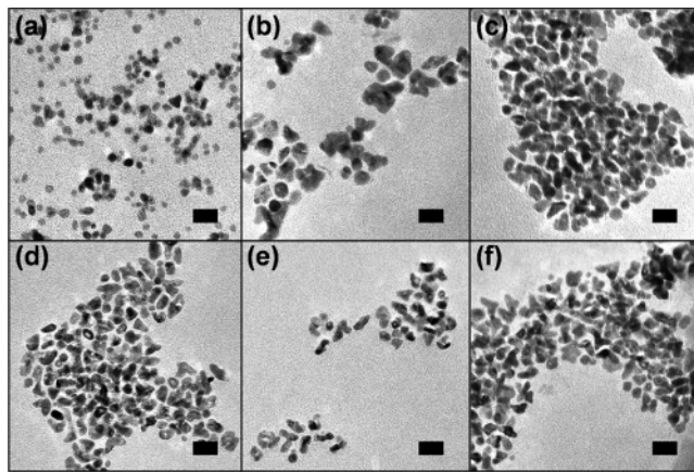
Figure 5. Rh 2 P multipods made with various cosolvents, injected, and aged for 1 h at 360 °C unless otherwise noted: (a) oleic acid; (b) octyl ether; (c) oleylamine; (d) ethanol + oleylamine (aged 15 min); (e) ethanol; (f) ethanol (aged at 340 °C). All scale bars are 20 nm.
