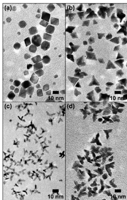
Figure 1. TEM images of Rh nanocrystals used as precursors: (a) cube derivatives (including cubes and octahedra); (b) triangle derivatives (including twinned and etched triangles); (c) thin-armed multipods; (d) thick-armed multipods.
