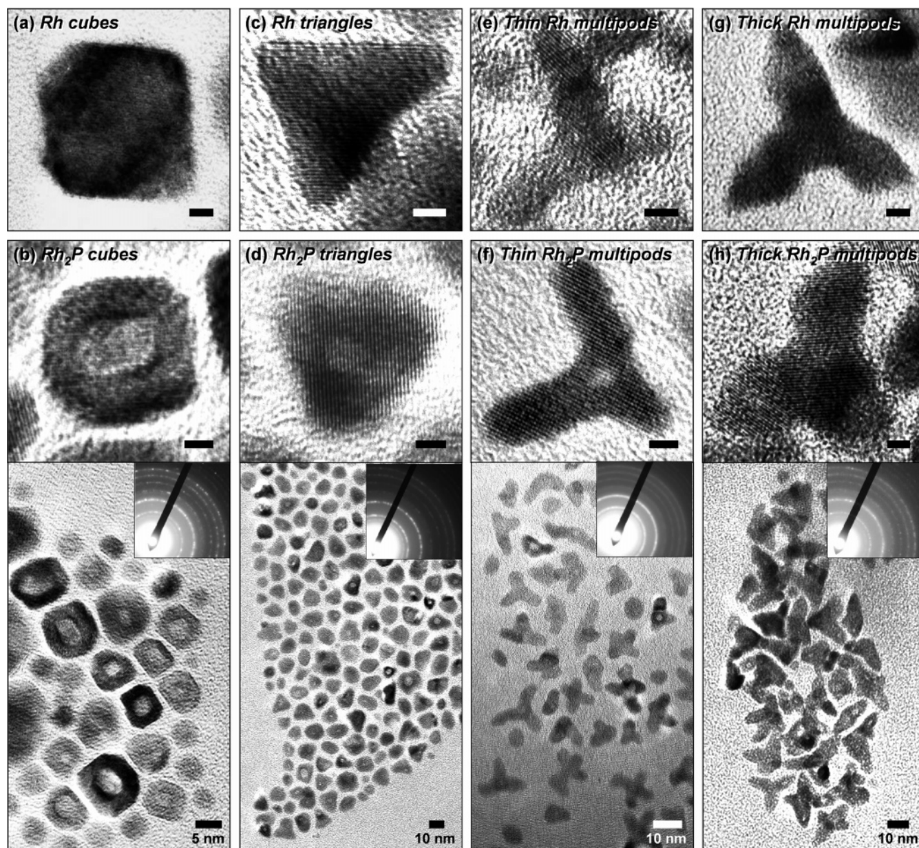
Figure 3. TEM images highlighting the shape-controlled conversion of Rh nanocrystal templates to \text{Rh}_2\text{P} : (a) Rh cube-derived nanocrystals and (b) \text{Rh}_2\text{P} formed from (a); (c) Rh triangle-derived nanocrystals and (d) \text{Rh}_2\text{P} triangles formed from (c); (e) thin-armed Rh multipods and (f) \text{Rh}_2\text{P} multipods formed from (e); (g) thick-armed Rh multipods and (h) \text{Rh}_2\text{P} multipods formed from (g). Scale bars are 2 nm unless otherwise labeled.
