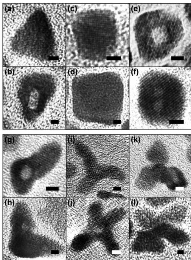
Figure 4. Representative Rh 2 P nanostructures obtainable by reaction of Rh nanocrystals with TOP: (a) solid triangle; (b) hollow triangle; (c, d) solid cubes; (e, f) hollow cubes; (g, h) fractured multipods; (i, j) multipods with hollow cores; (k, l) multipods with hollow arms. All scale bars are 2 nm.
