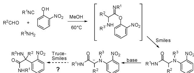
Scheme 1. Envisioned Smiles Cascades
