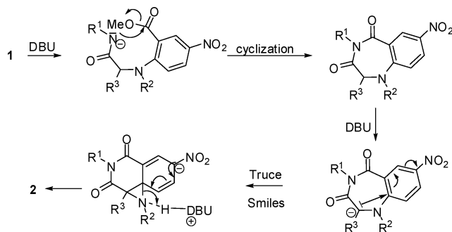
Scheme 4. Plausible Mechanism
