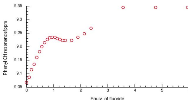
Fig. 4 NMR titration curve of compound 3 with fluoride anions in DMSO- d 6 -0.5% water.
