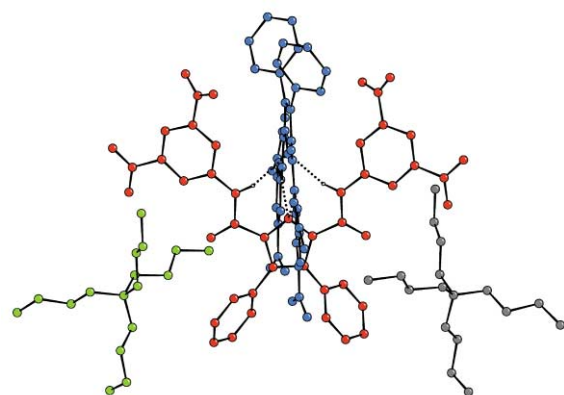
Fig. 7 The X-ray crystal structure of the tetrabutylammonium salt of 3- \text{H}^+ . Colours represent individual components of the assembly. Certain hydrogen atoms have been omitted for clarity.
