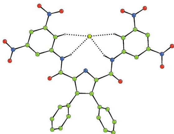
Fig. 5 The crystal structure of 3- \text{H}^+ binding chloride via NH and CH hydrogen bonds (two tetrabutylammonium counter cations have been omitted for clarity). Colour key: carbon = green, nitrogen = blue, oxygen = red, chloride = light green.
