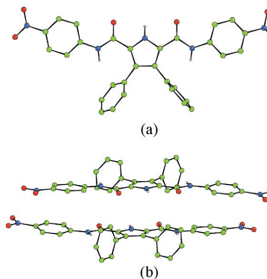
Fig. 1 (a) The crystal structure of compound 2 . Colour key: carbon = green, nitrogen = blue, oxygen = red. (b) Side view of the \pi -stacking interaction.
