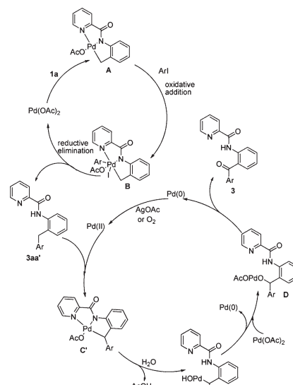
Scheme 2. Plausible Reaction Mechanism
