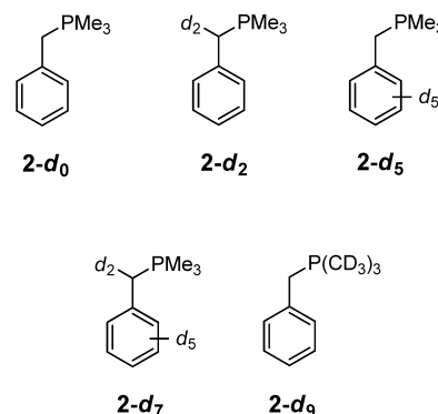
Chart 1. Benzyltrimethyl Phosphonium Isotopologues (2-d n )
