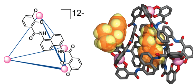
Figure 1. (Left) Schematic of host 1 with only one ligand shown for clarity. (Right) Solid-state structure of host 1 showing interior and exterior binding of \text{NMe}_3\text{Bn}^+ guest molecules (orange).
