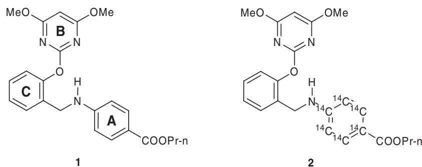
Figure 1. ZJ0273 (1) and propyl 4-(2-(4,6-dimethoxypyrimidin-2-yloxy)benzylamino)[phenyl- U - ^{14}\text{C}_6 ]benzoate (2).
