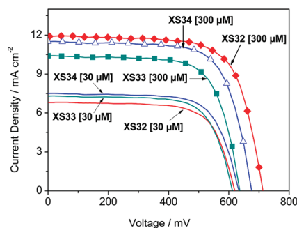
Figure 3. J – V curves of DSSCs based on the three dyes. Two different dye bath concentrations (300 and 30 \mu\text{M} ) were used for preparation of \text{TiO}_2 electrode.
