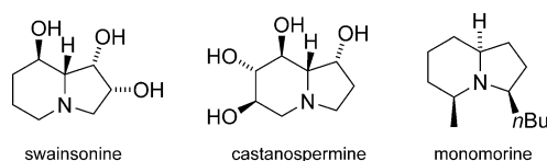
Scheme 1. Selected indolizidine natural products.
