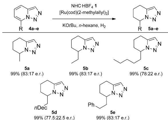
Scheme 4. Scope of the asymmetric hydrogenation of 1,2,3-triazolo-[1,5- a ]pyridines 4a–e . General conditions: [Ru(cod)(2-methylallyl) 2 ] (0.015 mmol), KOtBu (0.045 mmol), and 1 (0.03 mmol) were stirred at 70 °C in n -hexane (2 mL) for 12 h, after which the reaction mixture was added to 4a–e (0.30 mmol), and hydrogenation was performed at 100 bar and room temperature for 16 h. Yields of isolated products are given. Enantiomeric ratios were determined by HPLC on a chiral stationary phase.
