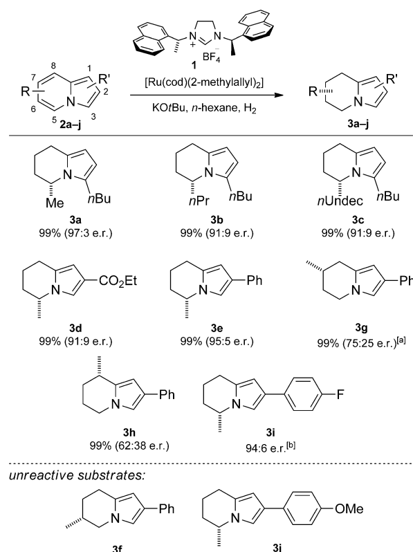
Scheme 3. Scope for the asymmetric hydrogenation of indolizines 2a–j . General conditions: [Ru(cod)(2-methylallyl)] 2 (0.015 mmol; cod = cyclooctadiene), KOtBu (0.045 mmol), and 1 (0.03 mmol) were stirred at 70 °C in n -hexane (2 mL) for 12 h, after which the reaction mixture was added to 2a–j (0.30 mmol), and hydrogenation was performed at 100 bar and room temperature for 24 h. Yields of isolated products are given. Enantiomeric ratios were determined by HPLC on a chiral stationary phase. The absolute configuration of 3a was determined by hydrogenation to monomorphine (see Scheme 5). [a] Reaction carried out at 100 bar and 40 °C. [b] 3i was obtained accompanied with over-reduction products and was impossible to purify for characterization.
