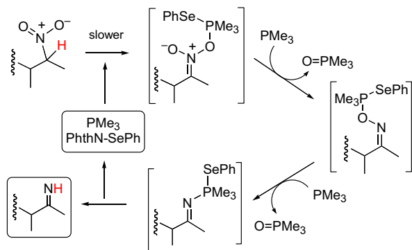
Scheme 3. Proposed mechanism for the reaction of nitro compounds with \text{PMe}_3/\text{PhthN-SePh} (Method B). Proton exchanges involving \text{PhthN}^-/\text{PhthNH} are not drawn (see the main text).
