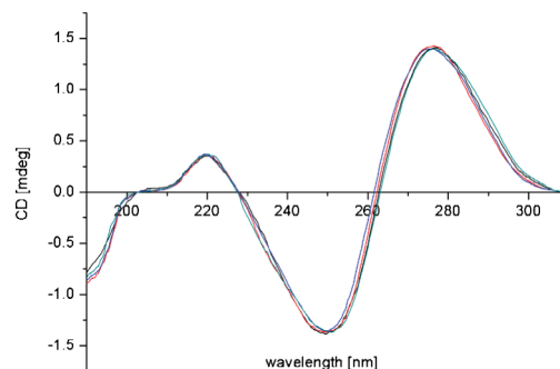
Fig. 4 CD-spectra of unmodified DNA (—), adamantane modified DNA (—), diamantane modified DNA (—) and triamantane modified DNA (—). The CD spectra show the characteristic profile of a B-DNA with a positive maximum at about 275 nm and a minimum at about 245 nm. Compared to the unmodified oligonucleotides the curve of the modified ones do not show significant differences.
