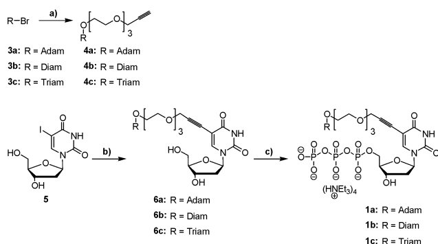
Scheme 1 a) 1- O -propargyl triethylene glycol, Et 3 N, 180 °C, 5 h, 4a : 83%, 4b : 76%, 4c : 79%; b) CuI, [Pd(PPh 3 ) 4 ], Et 3 N, 1- O -diamondoidyl-4- O -propargyl triethylene glycol 4 , DMF, rt, 24 h, 6a : 75%, 6b : 75%, 6c : 79%; c) proton sponge (1,8-bis(dimethylamino)naphthalene), POCl 3 , PO(OMe) 3 , 0 °C, then (Bu 3 NH) 2 H 2 P 2 O 7 , n Bu 3 N, then triethylammonium bicarbonate (TEAB) buffer, 1a : 6%, 1b : 5%, 1c : 5%.
