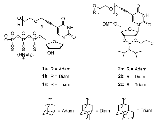
Fig. 2 Diamondoid modified triphosphates and phosphoramidites.
