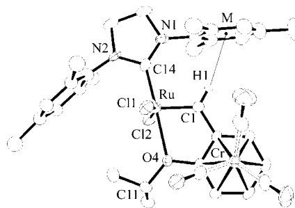
Figure 2. Structure of 11 in the crystal. Only one enantiomer is shown. Selected bond lengths [pm], angles [deg], and dihedral angles [deg]: Ru–C1 180.7(5), Ru–C14 195.9(6), Ru–O4 229.8(4), Ru–Cl1 231.8(2), Ru–Cl2 233.7(2), C14–N1 136.1(7), C14–N2 137.1(6), Cr–C2 224.9(6), Cr–C3 218.9(6), Cr–C4 218.6(7), Cr–C5 218.5(6), Cr–C6 222.9(6), Cr–C7 226.3(5); C1–Ru–O4 79.5(2), C1–Ru–C14 101.9(2), C14–Ru–O4 178.38(18), C11–Ru–Cl2 160.16(6); N1–C14–Ru–C1 3.5(6), N2–C14–Ru–C1 –177.8(5), C14–Ru–C1–C2 –179.3(5); C–H \cdots \pi hydrogen bond (M denotes the centroid of the mesityl substituent): C1 \cdots M 344.9, C1–H1 93, H1 \cdots M 253, C1–H1 \cdots M 170.
