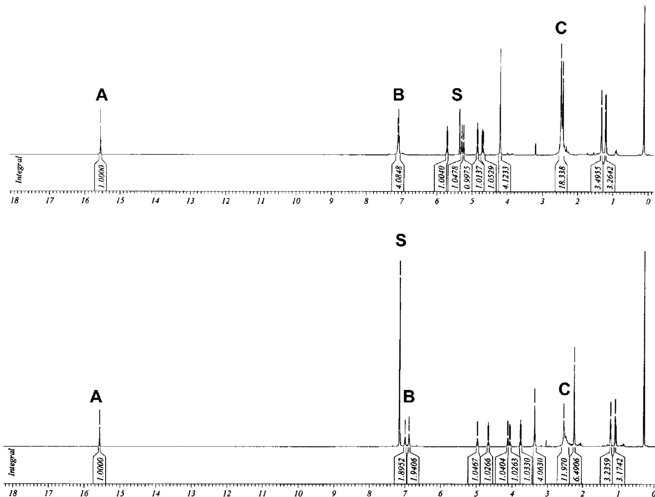
Figure 1. ^1\text{H} NMR spectra (400 MHz) of 11 in \text{CD}_2\text{Cl}_2 (top) and in \text{C}_6\text{D}_6 (bottom). Selected signal assignments: (A) benzylidene proton, (B) mesityl protons, (C) mesityl ortho -methyl protons, (S) residual solvent signal.
