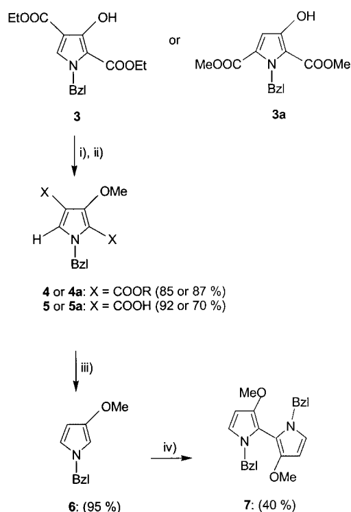
Scheme 1. i) \text{Me}_2\text{SO}_4 , acetone, \text{K}_2\text{CO}_3 , reflux; ii) \text{KOH} , \text{EtOH} ; iii) pyrolysis, 240^\circ\text{C} ; iv) \text{THF}/\text{Et}_2\text{O} , sec -BuLi, TMEDA, -60 to 0^\circ\text{C} , then \text{NiCl}_2 .
