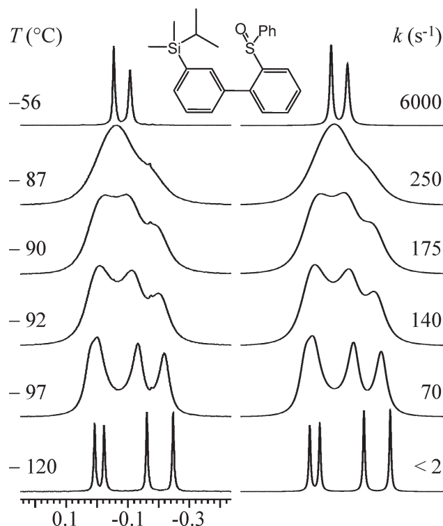
Fig. 2 Left: temperature dependence of the silicon bonded ^1\text{H} NMR methyl signals of ortho phenyl sulfoxide derivative 3 in \text{CHF}_2\text{Cl}/\text{CH}_2\text{FCl}_2 at 600 MHz. Right: line shape simulation obtained with the indicated rate constants.
