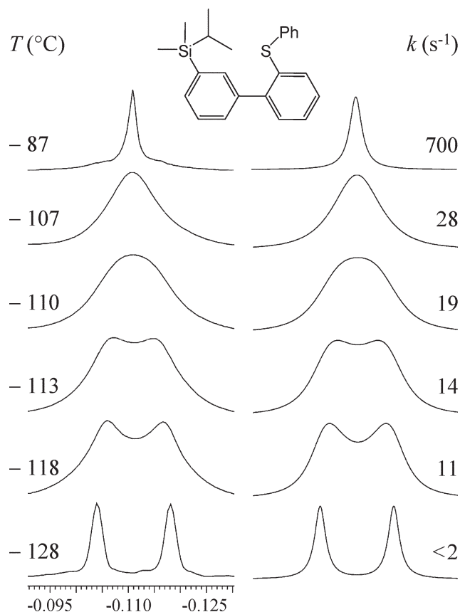
Fig. 1 Left: temperature dependence of the silicon bonded ^1\text{H} NMR methyl signal of ortho phenyl sulfide derivative 2 in \text{CHF}_2\text{Cl}/\text{CH}_2\text{FCl}_2 at 600 MHz. Right: line shape simulation obtained with the indicated rate constants.
