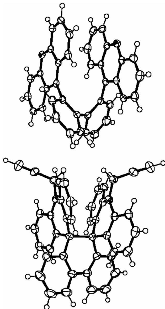
Fig. 1. X-ray structures of 5 (upper) and 4 (lower) measured at -120\text{ }^{\circ}\text{C} .
