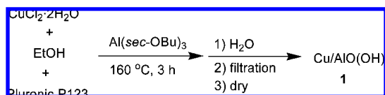
Scheme 1. Preparation of Catalyst
