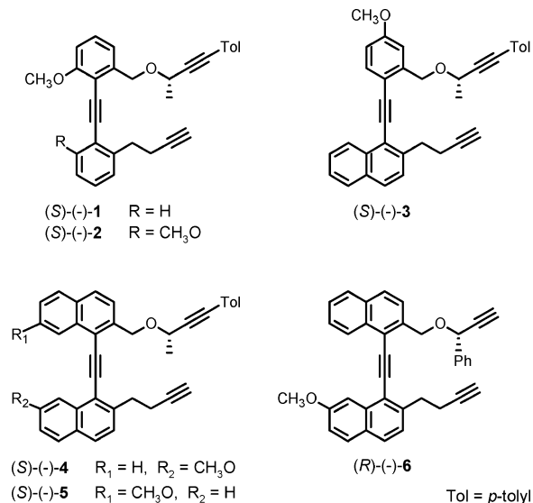
FIGURE 1. Model triynes for diastereoselective [2 + 2 + 2] cycloisomerization.
