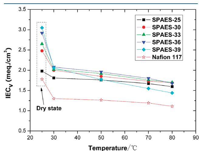
Figure 6. Volumetric IEC_v of SPAES-xx and Nafion 117 in water as a function of temperature.
