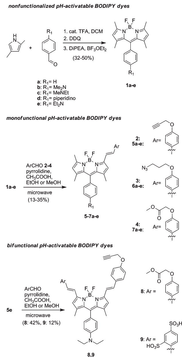
Scheme 1. Synthesis of Nonfunctionalized, Monofunctional, and Bifunctional BODIPY Dyes
