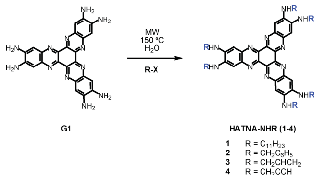
Fig. 1 Synthesis of the C_3 -symmetrical HATNA derivatives.
