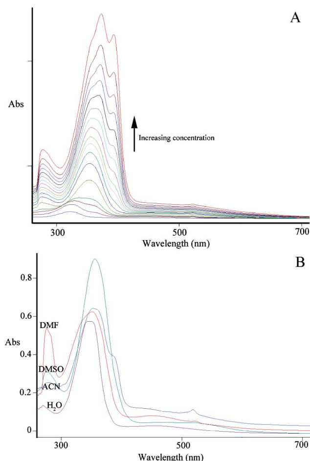
Fig. 5 UV-vis spectra of compound 1 ; (A) in solution and gel-state at different concentrations ( 10^{-5} – 10^{-3} M) and (B) in dilute solutions ( 10^{-5} mM) of solvents with different polarity (DMF, DMSO, acetonitrile-ACN, and H_2O ) at 25 °C.
