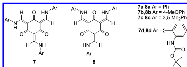
Figure 4. There are two possible geometric isomers of each compound 6a–d in its keto-enamine (NH) form, 7 and 8 , with symmetry C_{3h} and C_s , respectively.
