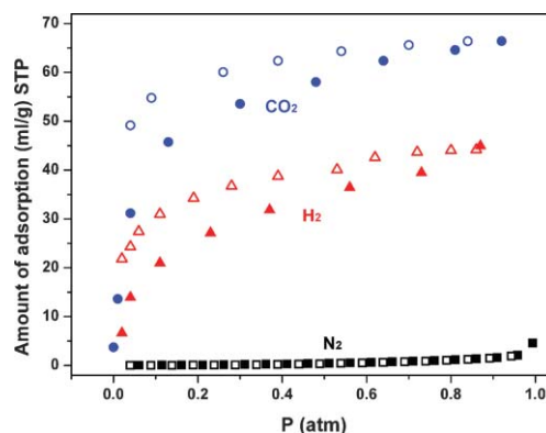
Fig. 4 Gas sorption isotherms of \text{N}_2 (77 K), \text{H}_2 (77 K) and \text{CO}_2 (195 K); ● and ○ represent the adsorption and desorption of \text{CO}_2 ; ▲ and △ \text{H}_2 , and ■ and □ \text{N}_2 , respectively.
