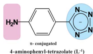
Scheme 1 4-Aminophenyl-1H-tetrazole (HL).
