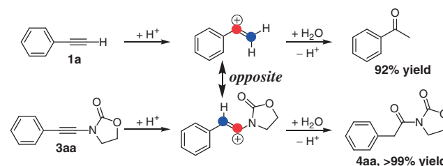
Scheme 2. The Sn–W mixed oxide-catalyzed hydration of 1a and 3aa . Yields were determined by gas chromatography using biphenyl as an internal standard. Reaction conditions for 3aa : 3aa (0.1 mmol), Sn–W mixed oxide (50 mg), \text{H}_2\text{O} (0.3 mmol), mesitylene (1 mL), 100 °C, under air (1 atm), 1 h. Reaction conditions for 1a : 1a (0.5 mmol), Sn–W mixed oxide (50 mg), \text{H}_2\text{O} (1 mmol), cyclooctane (2 mL), 100 °C, under air (1 atm), 1 h.
