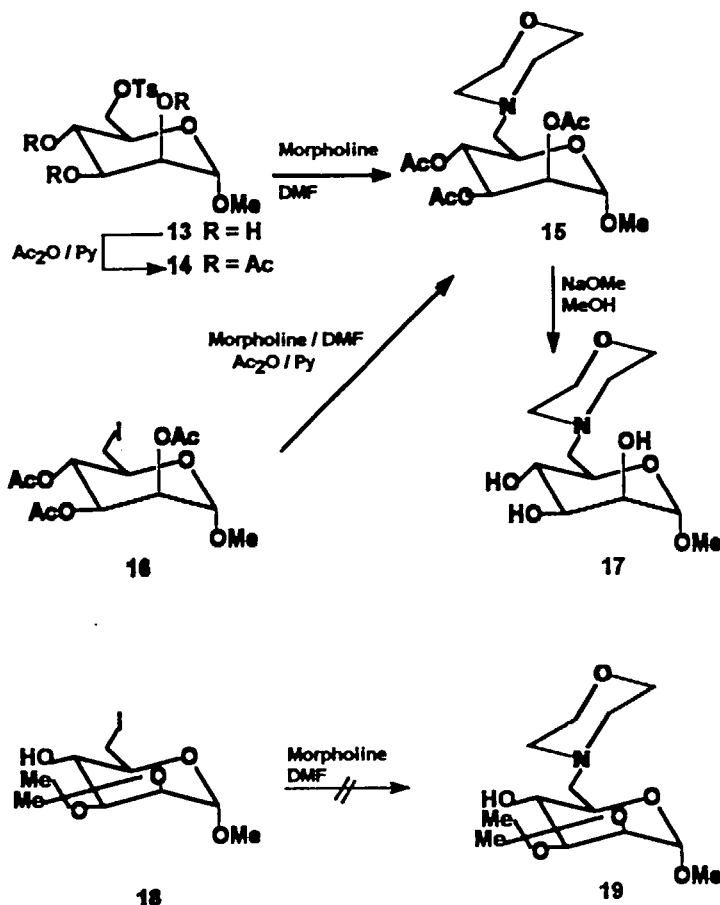
Scheme 3
