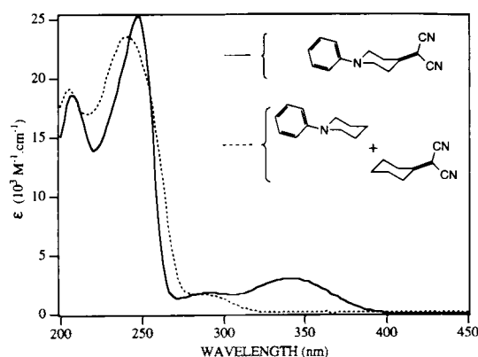
Fig. 1. UV-absorption spectrum of 14 (—) and sum spectrum of 1-phenylpiperidine and cyclohexylenepropanedinitrile (...) in n -hexane at 20°C.
