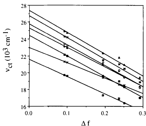
Fig. 3. Fluorescence maximum wavenumber \nu_{\text{ct}} ( 10^3 \text{ cm}^{-1} ) of series I (see Chart 3) vs. the \Delta f values of various solvents. R = phenyl (*), 4-methoxyphenyl (■), 4-methylphenyl (□) (offset + 1000 \text{cm}^{-1} ), 4-fluorophenyl (▲) (offset + 3000 \text{cm}^{-1} ), 3,5-dimethylphenyl (○) (offset + 2000 \text{cm}^{-1} ), 4-biphenyl (×), 2,4,6-trimethylphenyl (◆) (offset + 1000 \text{cm}^{-1} ).
