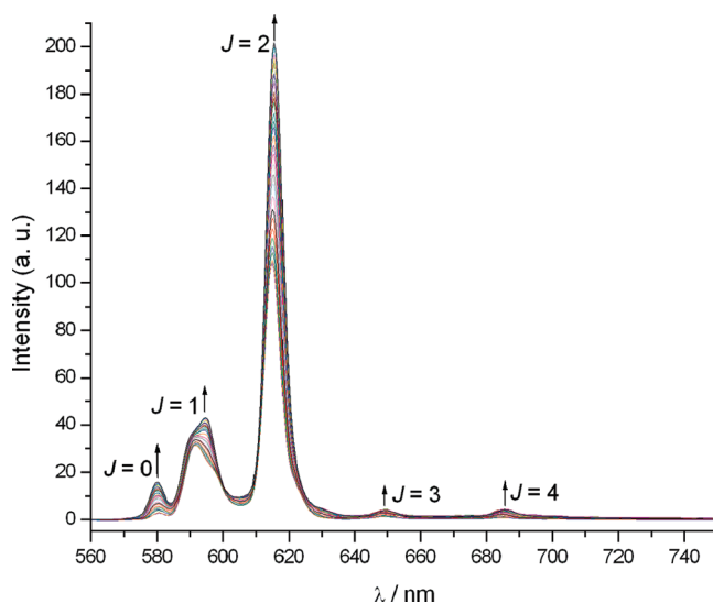
Figure 7. Variation of the emission spectrum for [\text{Eu}(\text{bp}12\text{c}4)(\text{H}_2\text{O})_9]^+ following addition of hydrogencarbonate [pH = 7.4 (HEPES), [complex] = ca. 10^{-5} M, \lambda_{\text{exc}} = 272 nm, I = 0.15 M NaCl].
