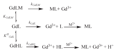
Scheme 1. Possible Reaction Pathways for the Dissociation of [\text{Gd}(\text{bp}12\text{c}4)]^+ in the Presence of a Divalent Metal Ion \text{M}^{2+}
