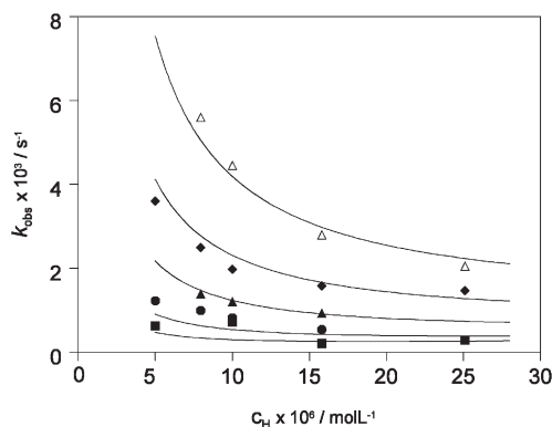
Figure 4. Plots of k_{\text{obs}} versus hydrogen ion concentration for the reaction between [\text{Gd}(\text{bp}12\text{c}4)]^+ and \text{Cu}^{2+} . C_{\text{Cu}} = 1 \text{ mM} (■), 2 \text{ mM} (●), 5 \text{ mM} (▲), 10 \text{ mM} (◆), and 20 \text{ mM} (△).
