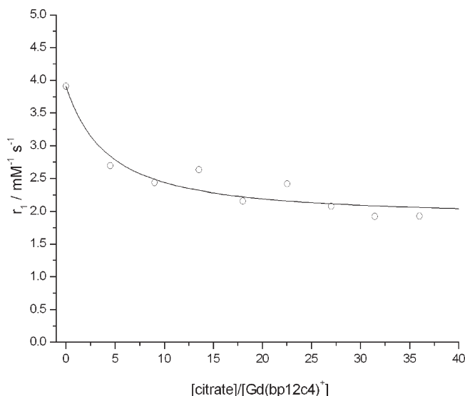
Figure 6. Relaxivity of [\text{Gd}(\text{bp}12\text{c}4)(\text{H}_2\text{O})_9]^+ ( \sim 1 mM) in the presence of increasing citrate concentration, at 500 MHz and 25 °C. The line is the fitted curve as explained in the text.
