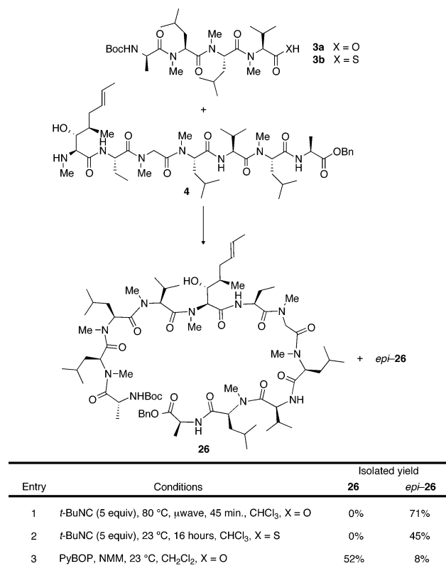
Scheme 7. Synthesis of Undeca peptide 26
