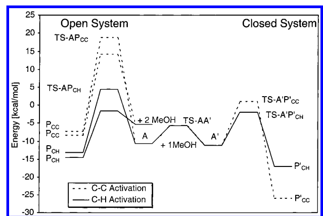
Figure 7. mPW1K/lanl2dz+p computed \Delta G_{298} reaction profiles for competing closed-arm and open-arm C–C and C–H activation routes with one and two MeOH spectator ligands.
