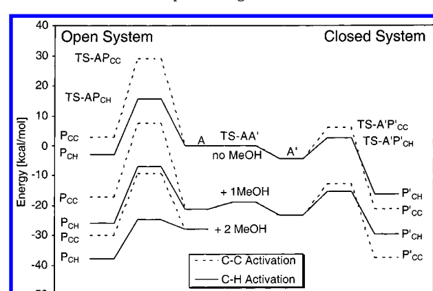
Figure 5. mPW1K/lanl2dz+p computed \Delta H_{298} reaction profiles for competing closed-arm and open-arm C-C and C-H activation routes with and without MeOH spectator ligands.
