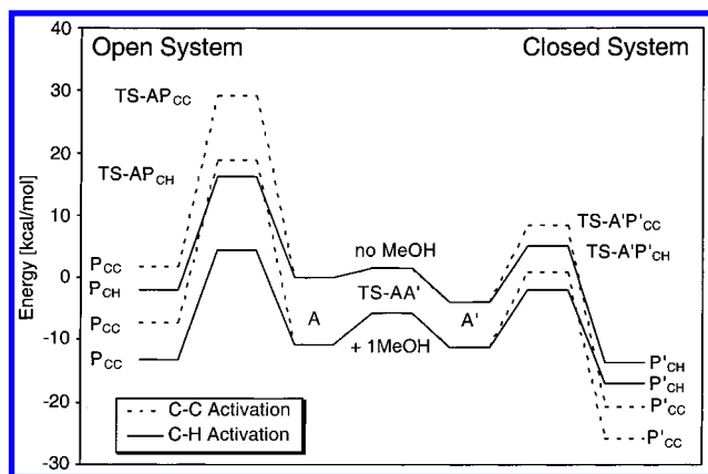
Figure 6. mPW1K/lanl2dz+p computed \Delta G_{298} reaction profiles for competing closed-arm and open-arm C–C and C–H activation routes with and without MeOH spectator ligands.
