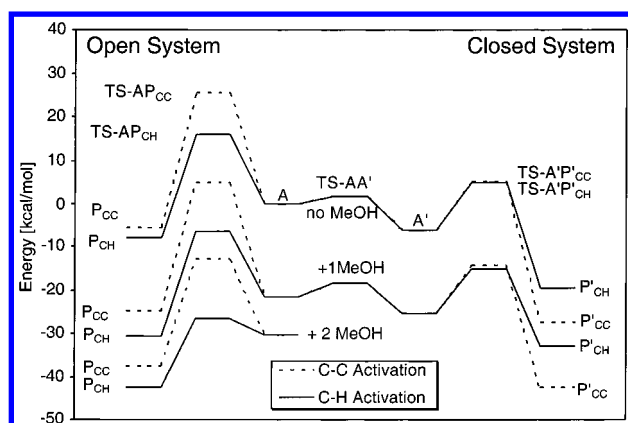
Figure 3. B3LYP/lanl2dz+p computed \Delta E_e reaction profiles for competing closed-arm and open-arm C-C and C-H activation routes with and without MeOH spectator ligands.
