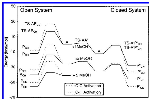
Figure 2. B3LYP/lanl2dz computed \Delta E_e reaction profiles for competing closed-arm and open-arm C-C and C-H activation routes with and without MeOH spectator ligands.
