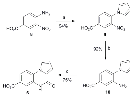
Scheme 2 Synthesis of lactam 6 . a) Dimethoxytetrahydrofuran, AcOH, 120 °C, 1 h; b) Pd/C, H 2 (1 atm), 1 : 1 EtOAc/MeOH, 14 h; c) triphosgene, toluene, reflux, 4 h.
