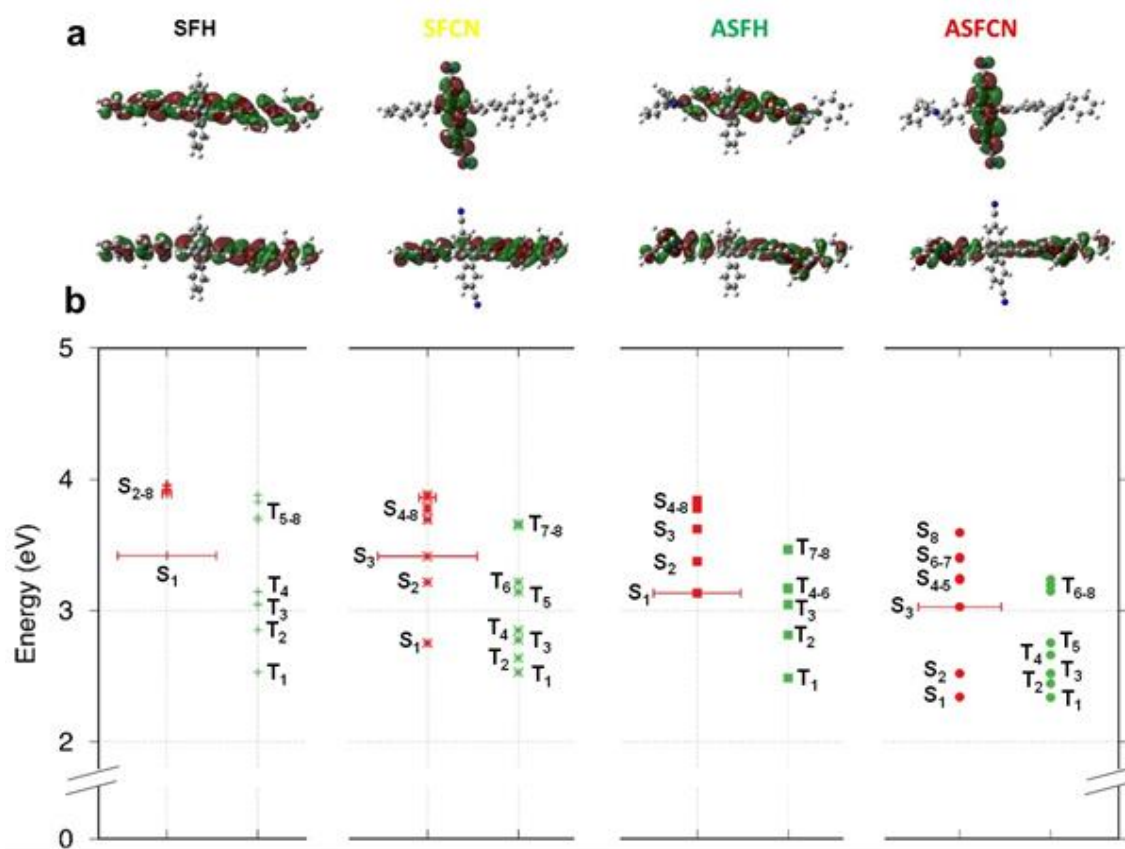
Figure 6. Electronic structure of model oligomers. (a) HOMO (bottom) and LUMO (top) of model trimers calculated using B3LYP/6-311g*. The D-oA motif results in complete localisation of the LUMO on the orthogonal fluorene unit. (b) Singlet and triplet states calculated by linear-response time-dependent density-functional-theory (LR-TD-DFT) at B3LYP/6-311g*. The width of the state indicates the absorption oscillator strength, plotted logarithmically, indicating the large Pi-Pi* transition which will dominate optical absorption. The numbering is by order of energy, separately for both singlet and triplet states.
