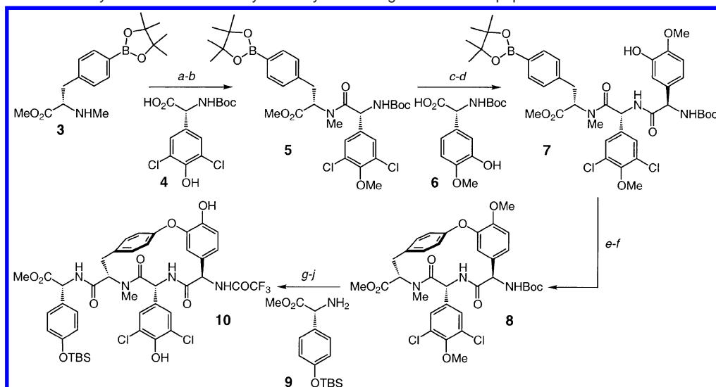
Scheme 2. Enantioselective Synthesis of the Macrocyclic Biaryl Ether Segment of Chloropeptins a
