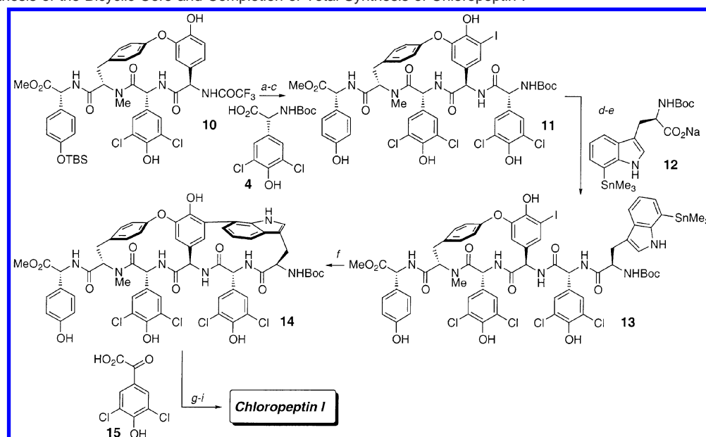
Scheme 4. Synthesis of the Bicyclic Core and Completion of Total Synthesis of Chloropeptin I a
