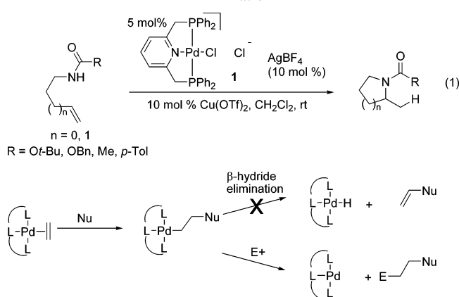
Scheme 1. Hydroamination via Inhibition of \beta -hydride Elimination
