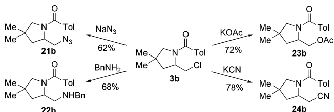
Scheme 2. Nucleophilic Substitutions
