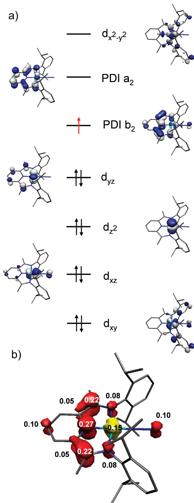
Figure 4. (a) Qualitative molecular orbital diagram for [(iPrPDI)CoN_2] computed from a B3LYP DFT calculation. (b) Spin density plot obtained from a Mulliken population analysis. Positive spin density is shown in red, and negative spin density is shown in yellow. The coordinate system is defined as “z” perpendicular to the idealized square plane of the molecule and “x” along the Co–N≡N vector.
