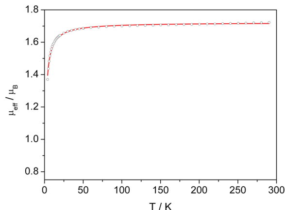
Figure 1. Temperature-dependent SQUID magnetization data (1 T) for samples of ( ^{\text{iPr}}\text{PDI})\text{CoN}_2 plotted as a function of the magnetic moment ( \mu_{\text{eff}} ) vs temperature ( T ). The data are corrected for underlying diamagnetism.
