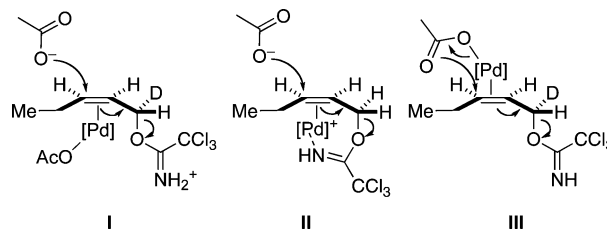
Figure 4. Three reaction pathways investigated.
