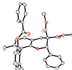
X-ray structure of 22a . Hydrogen atoms are omitted for clarity.
