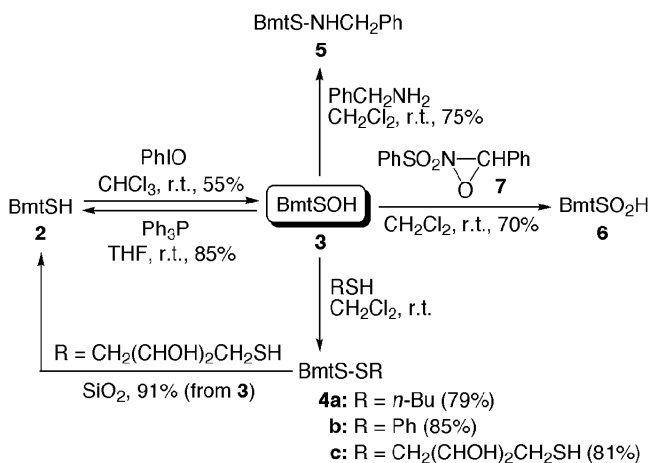
SCHEME 2 Synthesis and reactions of BmtSOH ( 3 ).
