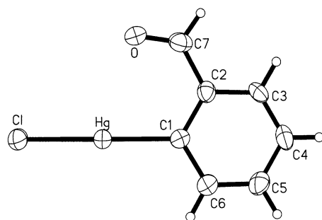
Fig. 1. Molecular geometry of \text{Hg}[\text{C}_6\text{H}_4(\text{CHO})\text{-}2]\text{Cl} ( 2 ).
