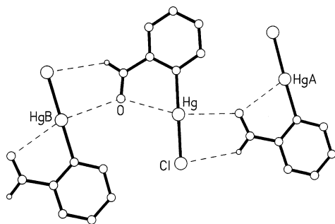
Fig. 2. Section of chain in the crystal of Hg[C 6 H 4 (CHO)-2]Cl ( 2 ).
