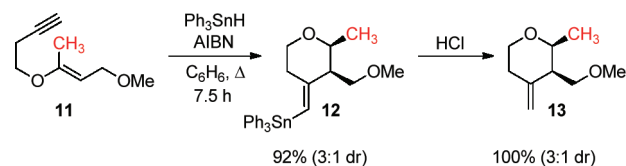
Scheme 1. Radical Cyclization onto a Mono-Vinyl Ether
