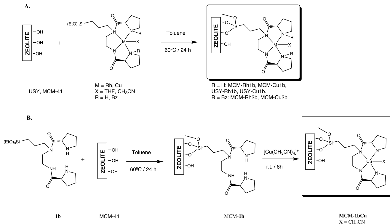
Scheme 2. Preparation of heterogenised complexes: Route A or B.
