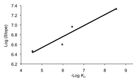
Figure 4. Correlation between literature-reported binding constants and slopes. 9 Data from Figure 3a (see Table S1).
