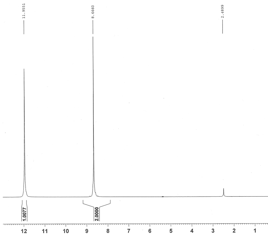
Fig. 3 ^1\text{H} NMR spectrum of \{[\text{SO}_3\text{H-Pyrazine-SO}_3\text{H}]\text{Cl}_2\}
