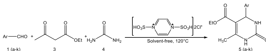
Scheme 2 Synthesis of DHPMs catalyzed by \{[\text{SO}_3\text{H-Pyrazine-SO}_3\text{H}]\text{Cl}_2\} under solvent-free conditions
