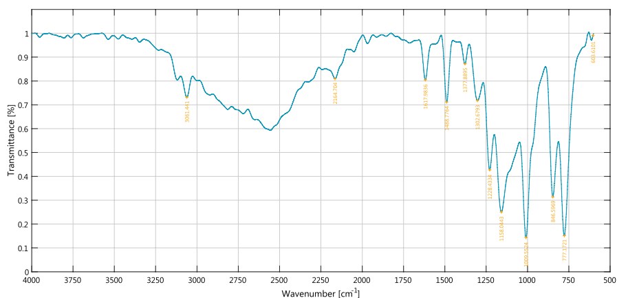
Fig. 2 FTIR spectrum of \{[\text{SO}_3\text{H-Pyrazine-SO}_3\text{H}]\text{Cl}_2\}
