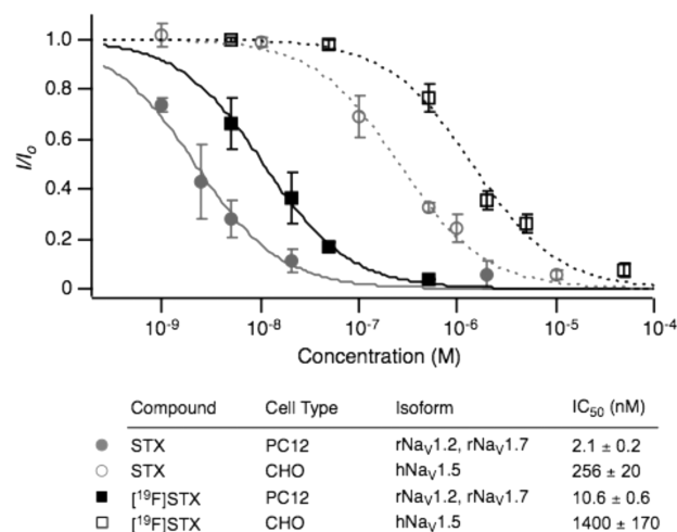
Figure 1. Concentration–response curves and \text{IC}_{50} values for STX (circles) and [ ^{19}\text{F} ]STX (squares) tested against differentiated PC12 cells endogenously expressing TTX-sensitive \text{Na}_v 1.2 and \text{Na}_v 1.7 (filled), and CHO cells transiently expressing TTX-insensitive \text{Na}_v 1.5 (hollow) [ n \geq 3 , error bars represent standard deviations; I/I_0 = remaining current/initial current]. Current versus time plots are shown in Figure S2 in the Supporting Information.
