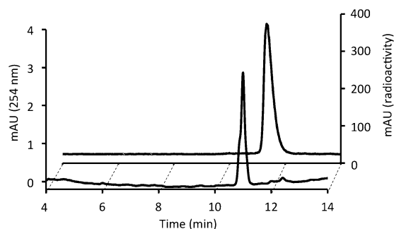
Figure 2. Analytical HPLC chromatogram of formulated [ ^{18}\text{F} ]STX coinjected with [ ^{19}\text{F} ]STX.
