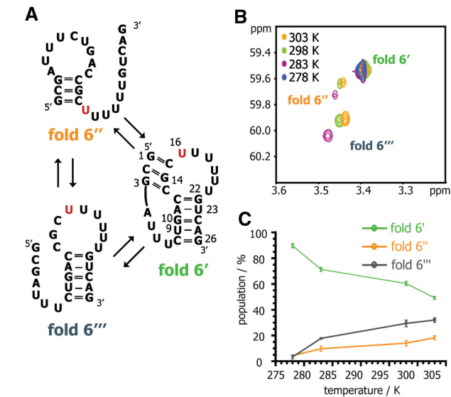
Figure 3. Temperature dependence of folding state populations of RNA sequence 6. (A) Representation of the three possible folding states. The red U denotes the 2'-O- 13 CH 3 -uridine label. (B) 1 H, 13 C-HSQC spectra of RNA sequence 6 at various temperatures ranging from 278 to 303 K. (C) Folding state populations (in %) versus temperature. The populations were determined as the mean value from three independent HSQC measurements at the indicated temperature (error bars from standard deviation). Conditions: 0.75 mM RNA, 2.5 mM MgCl 2 , 50 mM sodium phosphate, pH 6.5, H 2 O/D 2 O 9/1, 298 K.
