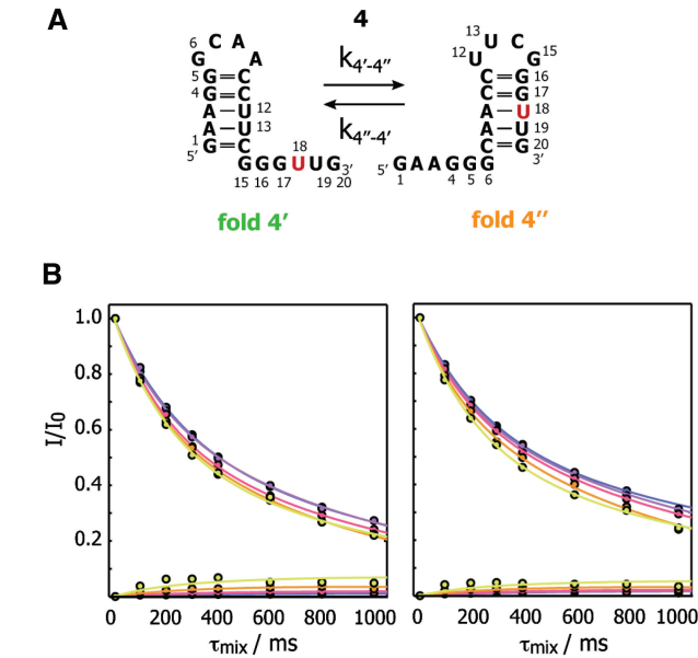
Figure 4. Kinetics of sequence 4 analyzed by 13 C longitudinal exchange spectroscopy. (A) Interconversion between conformations 4' and 4''. The uridine nucleotide that serves as a sensor is highlighted in red. (B) Signal intensities as a function of mixing time are shown for a set of temperatures. The left panel shows normalized intensities of the correlation peak of conformation 4' and the exchange peak corresponding to transition 4' → 4''. The right panel depicts the intensities of the correlation peak of conformation 4'' and the exchange peak corresponding to transition 4'' → 4'. Experiments performed at different temperatures are color-coded (298 K: blue, 300 K: magenta, 303 K: red, 306 K: orange, 310 K: yellow).
