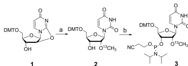
Scheme 1. Synthesis of the 2'- O - ^{13}\text{CH}_3 -uridine phosphoramidite 3 ; (a) 6 eq. ^{13}\text{C} -magnesium methoxide [ \text{Mg}(\text{O}^{13}\text{CH}_3)_2 , freshly prepared from magnesium turnings and ^{13}\text{CH}_3\text{OH} ] in anhydrous dimethylformamide, 100^\circ\text{C} , 2 h, 93%; (b) 1.5 eq. (2-cyanoethyl)- N , N -diisopropylchlorophosphoramidite, 10 eq. N -ethyltrimethylamine in anhydrous dichloromethane, room temperature, 2.5 h, 71%.
