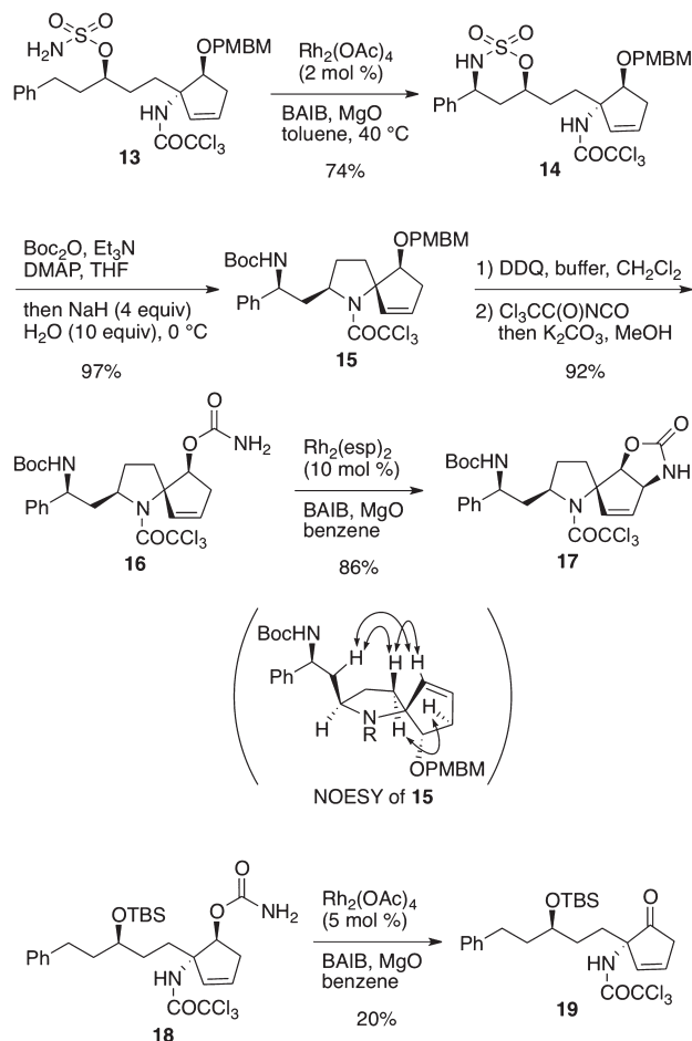
Scheme 3. Preparation of Key Intermediate 17
