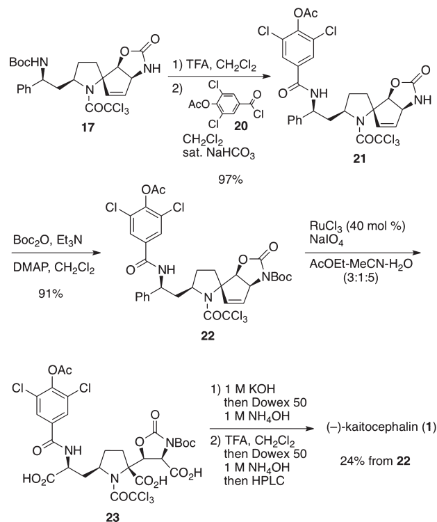
Scheme 4. Synthesis of (–)-Kaitocephalin
