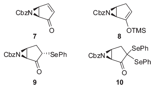
Figure 1. Enone 7 and enone's precursors 8 – 10 .
