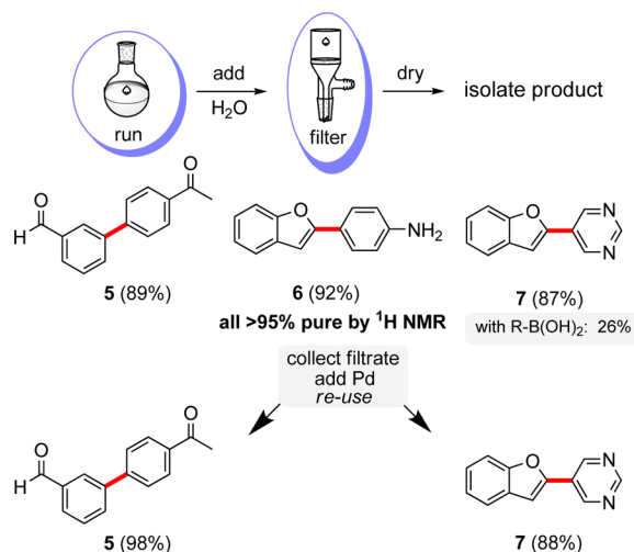
Scheme 4. Sequence for Organic Solvent-Free Suzuki–Miyaura Reactions: Couple/Filter/Recycle
